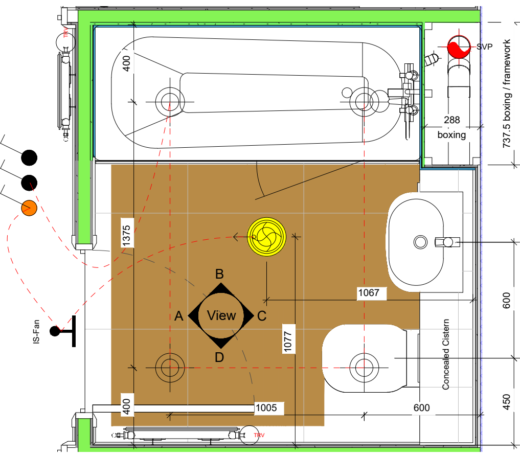
1 Bathroom Layout 1 : 20
