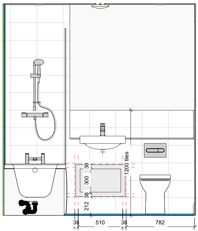
C Bathroom - View C 1 : 25
